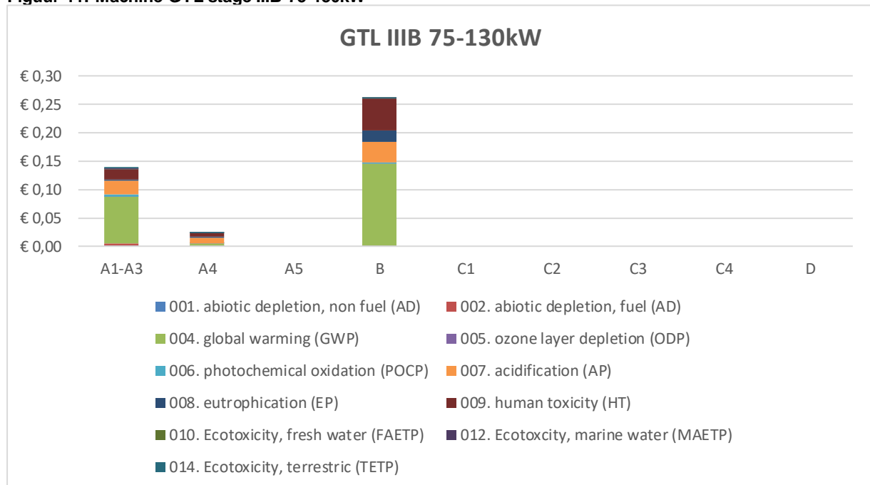
Figuur 11: Machine GTL stage IIIB 75-130kW
